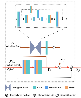
Figure 4.6: FAU architecture. Extracted from Chen et al. (2021a).
