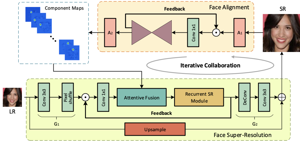
Figure 4.2: DICNet architecture. Extracted from Ma et al. (2020).
