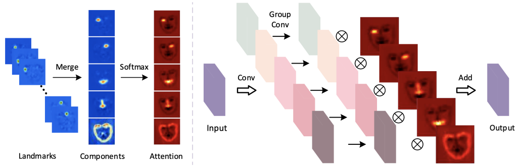
Figure 4.3: Landmark heatmap-extraction process. Extracted from Ma et al. (2020).
