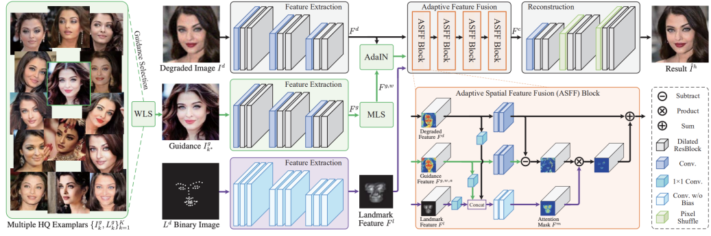
Figure 4.4: ASFFNet architecture. Extracted from Li et al. (2020).
