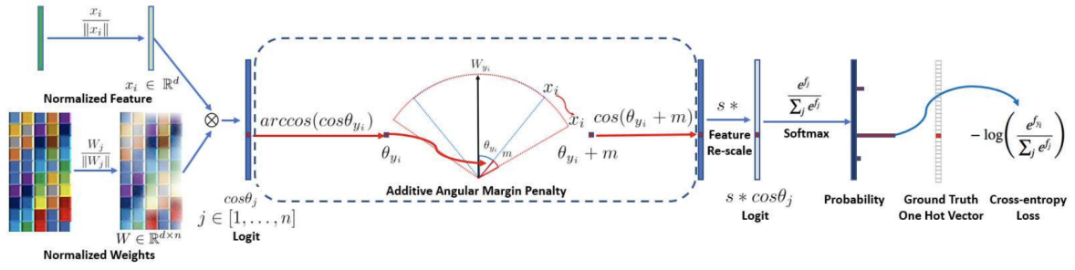
Figure 4.7: ArcFace architecture. Extracted from Deng et al. (2019).
