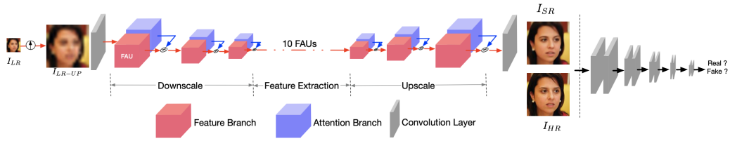
Figure 4.5: SPARNet architecture. Extracted from Chen et al. (2021a).
