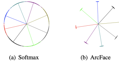
Figure 4.8: ArcFace geometric interpretation. Extracted from Deng et al. (2019).
