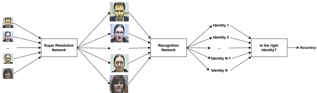
Figure 4.1: Proposed evaluation pipeline.
